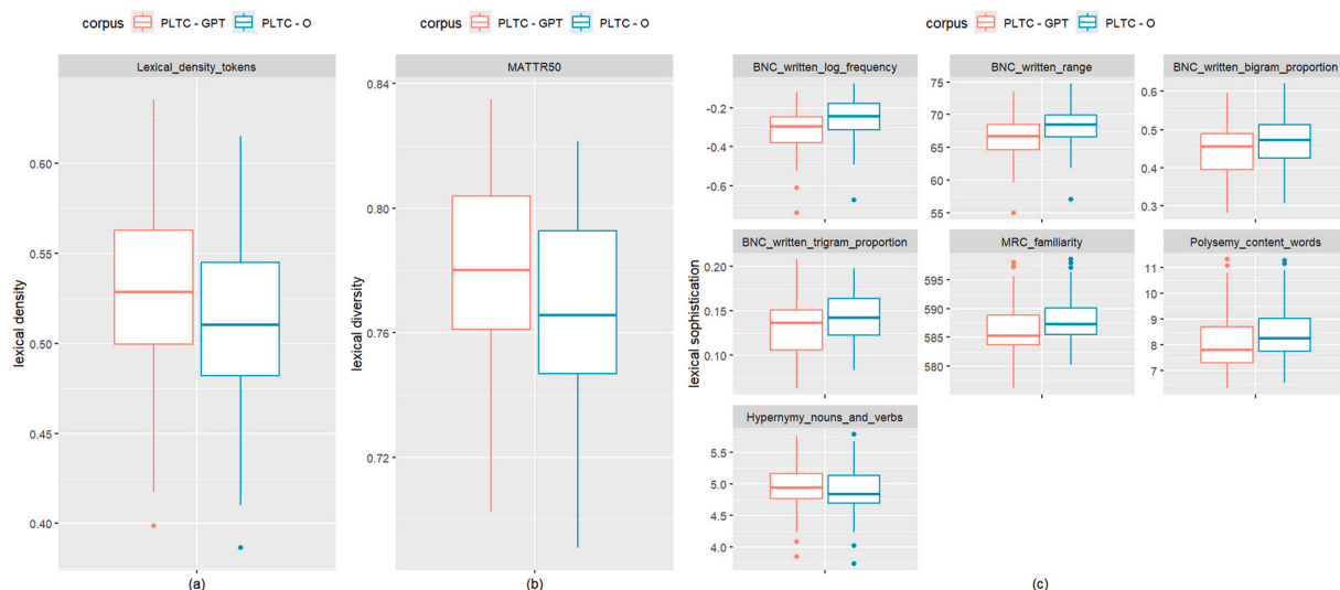
Fig. 2. Lexical complexity feature scores between the two corpora: (a) lexical density; (b) diversity; (c) sophistication.
